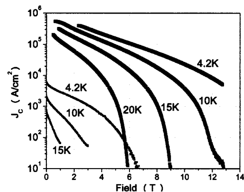
FIG. 3. Magnetization J_c(H, T) values derived for X=0.0525 (thick lines) and X=0.17 (narrow lines). Comparison of the fields at which J_c tends to zero are about half the values of H_{c2}(T) found in Fig. 1.
