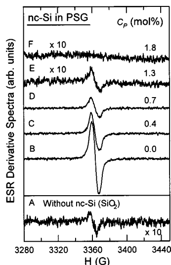
FIG. 3. ESR derivative spectra of a SiO 2 film (A), and SiO 2 (B) and PSG (C)–(F) films containing nc-Si. For the samples containing nc-Si, the size and concentration of nc-Si are fixed to almost the same and C_P is changed from 0 to 1.8 mol %.
