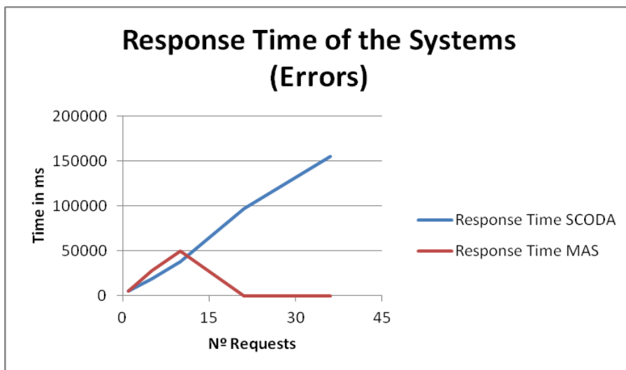
Figure 6. Graphic Detail of response (ms) on simultaneous requests for a MAS and SCODA with errors
