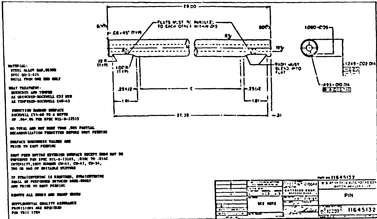
Figure 2.1. Regular Production (As Received) Tank Track Pin
