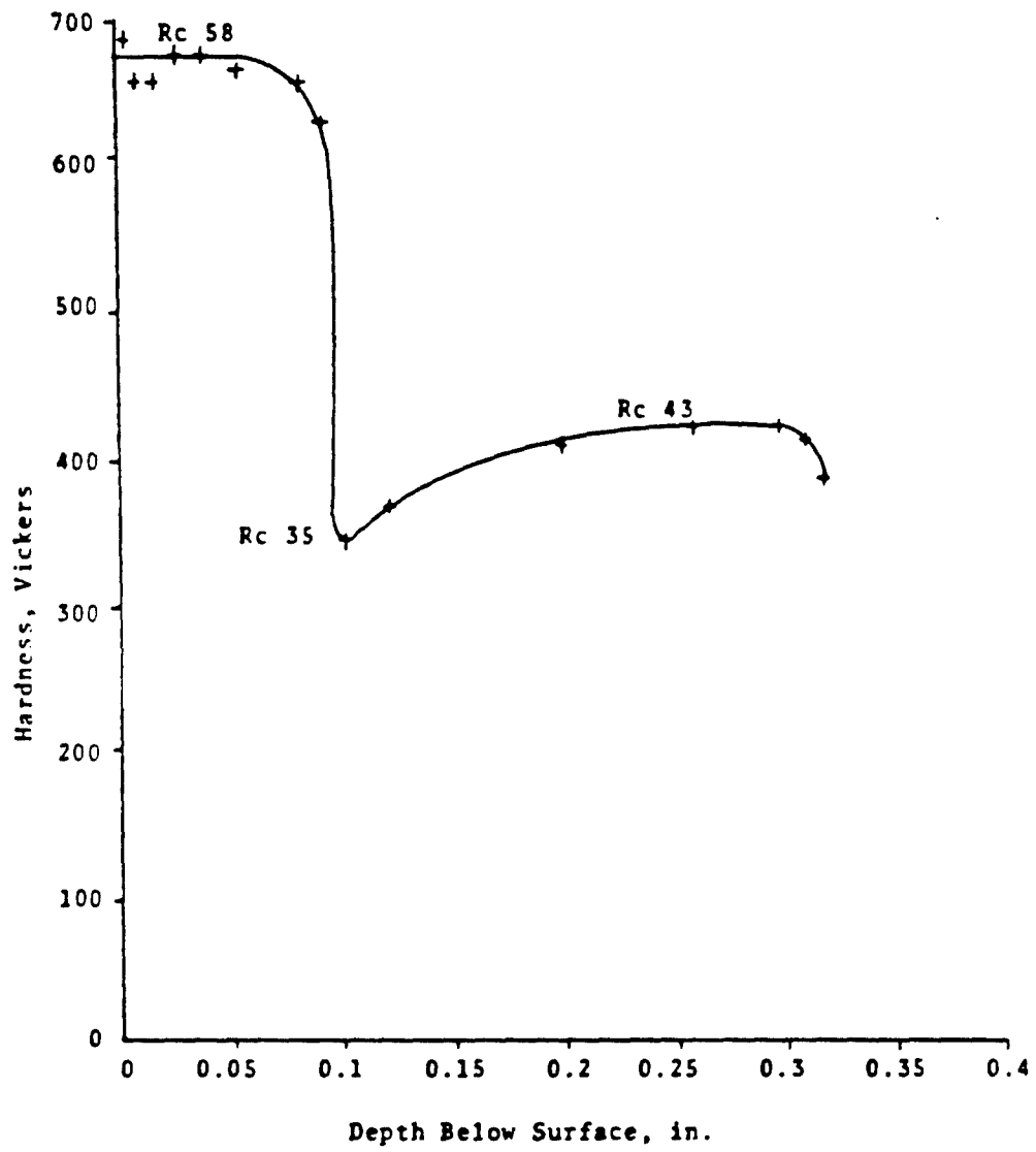
Figure 5-29. Hardness Profile of Stress Shot Peened 8650H Pin.
