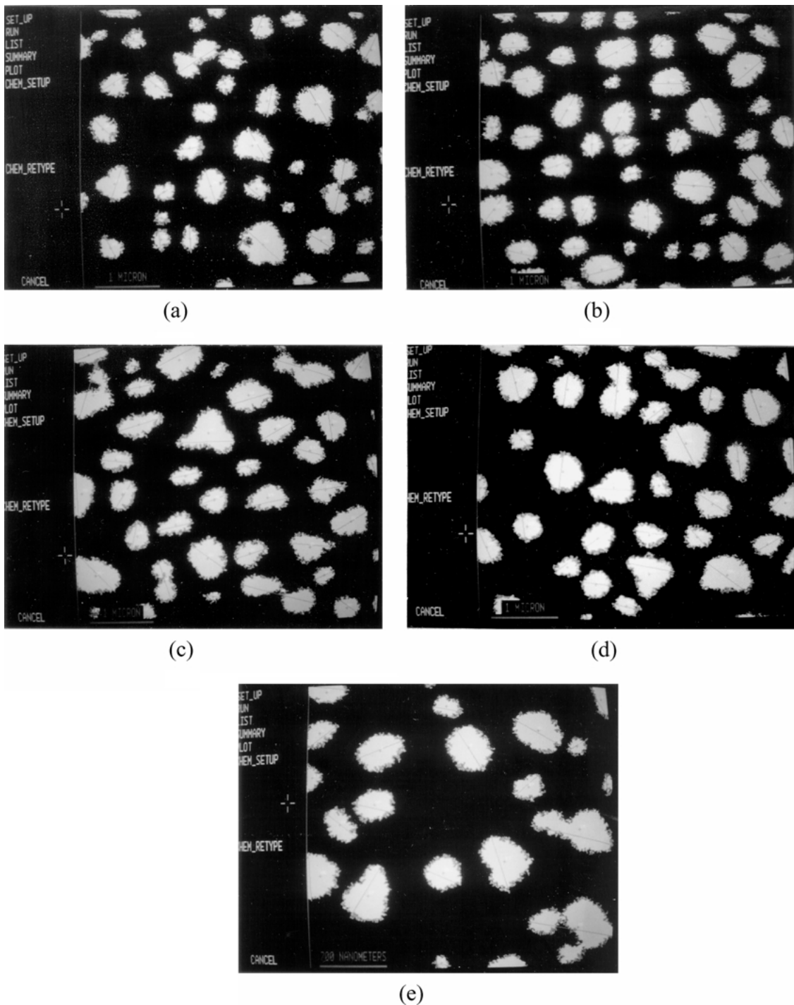
Figure 10 Microstructure images obtained by electron image analyzer after salt bath aging at: (a) 700°C (b) 750°C (c) 800°C and (d) 850°C for 60 min., and normal aging at: (e) 850°C for 240 min.( \times 15000 ).
