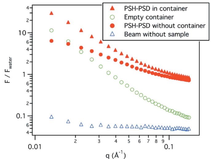
Figure 3 Ratio F/F_{water} of scattering functions of different samples to that of 1 mm-thick layer of water versus scattering vector q . Full triangles: 0.5 mm-thick solid sample made of 2% (v/v) deuterated polystyrene (PSD) and 98% (v/v) non-deuterated polystyrene (PSH) in a 3 mm-thick Al alloy container. Hollow circles: empty container. Full circles: solid sample alone. Hollow triangles: beam without sample. Measurements performed on PACE (LLB) at \lambda = 6 Å, D = 2.38 m. Statistical error bars are smaller than the data symbols.
