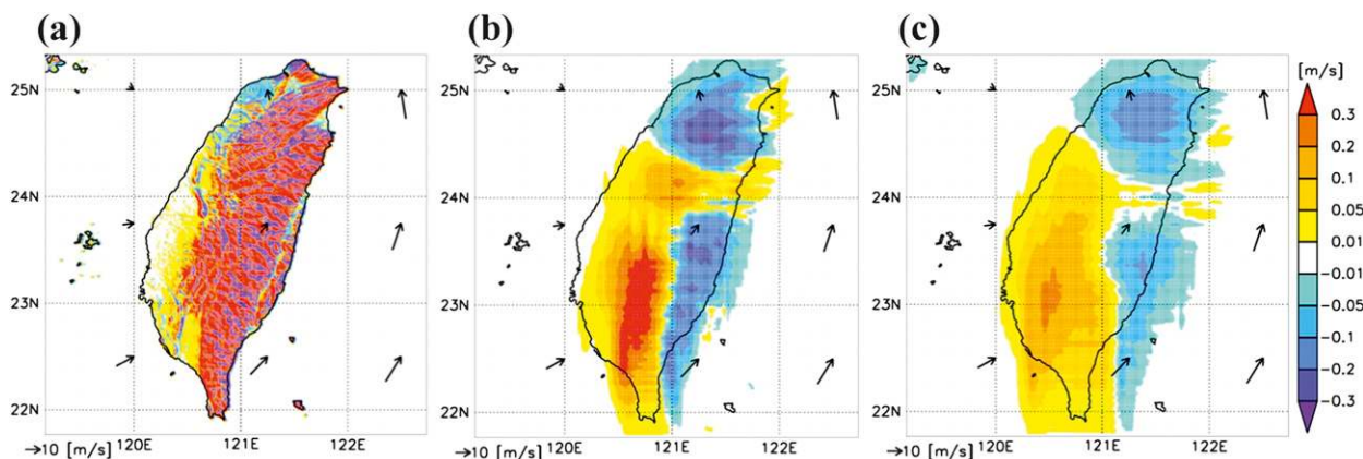
FIG. 4. Orographically forced upward motion w_{oro} ( \text{m s}^{-1} ) over Taiwan area estimated using Eq. (1) with surface wind data from JCDAS at 1800 UTC 8 Aug 2009 and SRTM30 data: (a) original, 1 km, and averaged within the horizontal length scale of (b) 50 km and (c) 100 km. Vectors are JCDAS surface wind ( \text{m s}^{-1} ).
