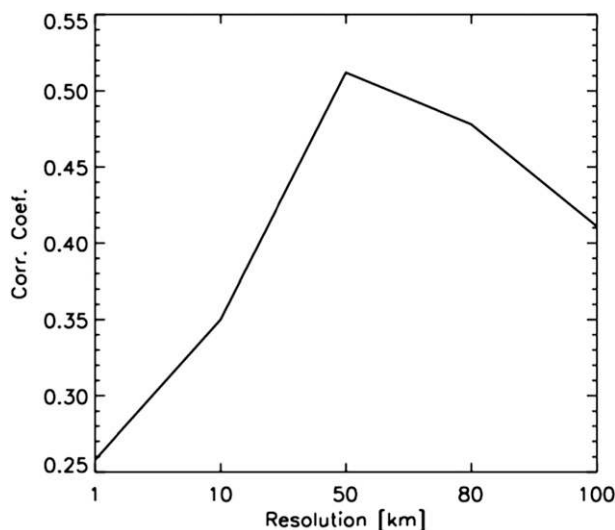
FIG. 5. Correlation coefficients between PR 2A25 near-surface rain shown in Fig. 1b and w_{oro} estimated using elevation data with five horizontal resolutions (1, 10, 50, 80, and 100 km). Calculations for correlation coefficients were made only for the upward motion regions.
