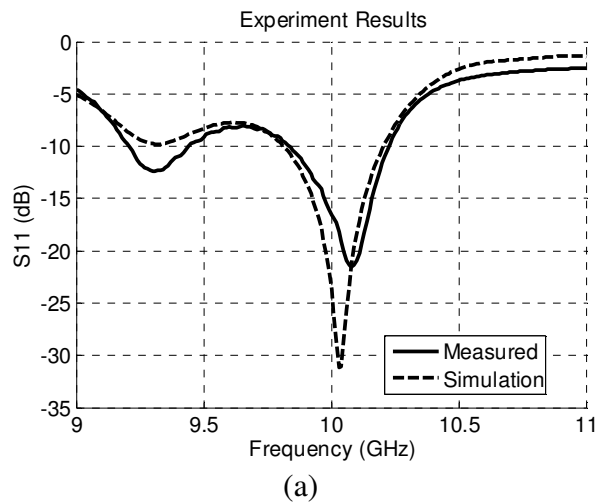
Fig. 3. Simulation and measured results of the antenna shown in Fig. 2(a); (a) return loss and far-field pattern at 10GHz in (b) E-plane and (c) H-plane
