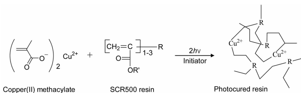
Scheme 1. Molecular structures of metal complex and the conceptual scheme of the two-photon polymerization with SCR500 resin.
