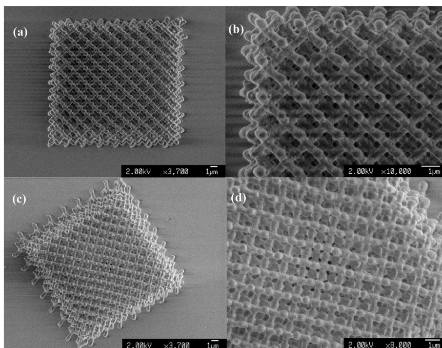
Figure 1. Scanning electron microscopy (SEM) images of two-photon polymerized 3D diamond photonic crystals containing photopolymerizable oligomers doped with Cu 2+ : (a) Top view and (b) magnified image of the 8 × 8 × 2 lattice before heating. (c) Top view and (d) magnified image of the 8 × 8 × 5 lattice after heating.
