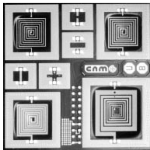
Fig. 12. Top-view photograph of the IC designed to test the inductor's layout optimization method. Three constant strip-width inductors are integrated together with the optimized layout. Some test structures are also included to allow pad deembedding purposes.
