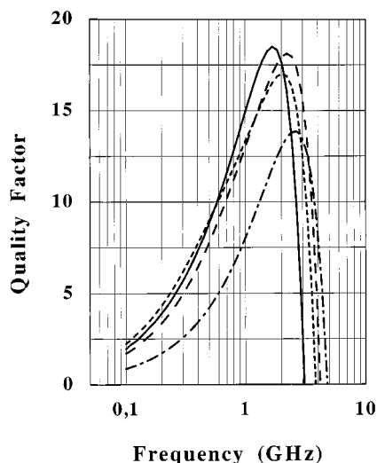
Fig. 14. Simulated Q factors as a function of frequency for the inductor structures on Fig. 12. (---) corresponds to the inductor performed using a metal strip 16\text{-}\mu\text{m} wide, (- - -) 36\text{-}\mu\text{m} , (- - - - -) 51\text{-}\mu\text{m} , and (—) optimized layout.
