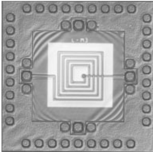
Fig. 1. Top-view photograph of a four-and-one-half-turn square spiral RF integrated inductor, performed using silicon-based MCM technology, complemented with silicon micromachining postprocessing. The light square in the center corresponds to the area where silicon has been removed.
