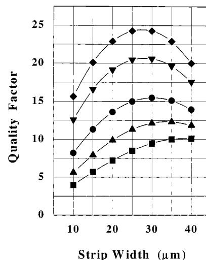
Fig. 9. Q factor as a function of the metal strip width for different 20-nH RF integrated inductors. ■ are the obtained Q factors at 0.7-GHz frequency of operation, ▲ 1 GHz, ● 1.5 GHz, ▼ 2.5 GHz, and ◆ 3.5 GHz.
