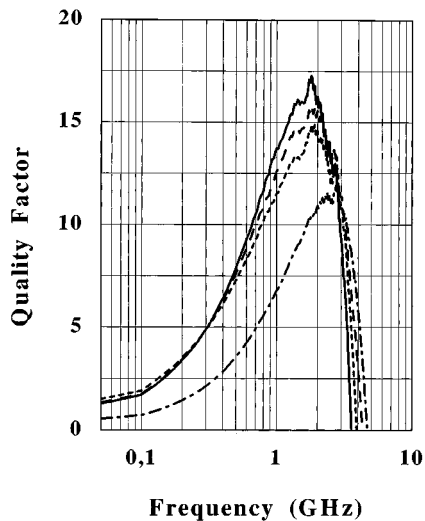
Fig. 13. Experimental Q factors as a function of frequency for the inductor structures on Fig. 12. (---) corresponds to the inductor performed using a metal strip 16\text{-}\mu\text{m} wide, (- - -) 36\text{-}\mu\text{m} , (- - - - -) 51\text{-}\mu\text{m} , and (—) optimized layout.
