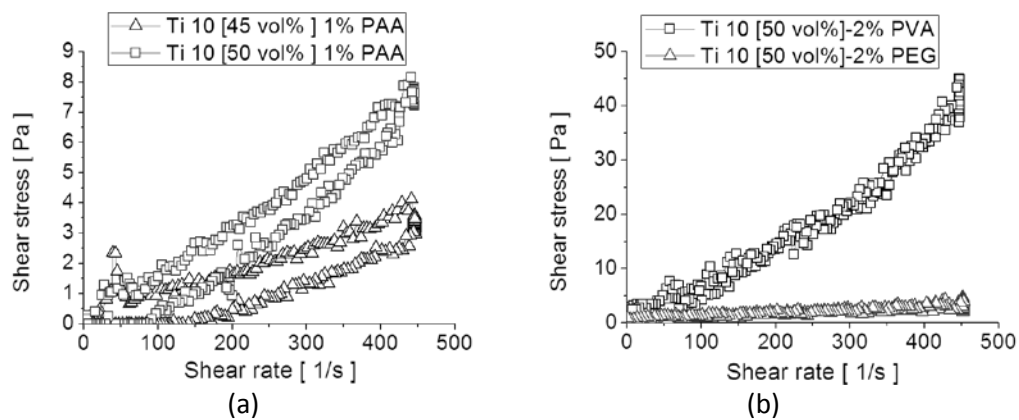
Figure 2- a) Flow curve for slurries of Ti10 for different solid contents b) Flow curves for Ti10 slurry with PVA and PEG.
