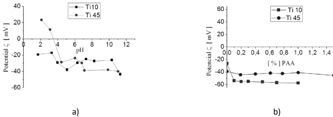
Figure 1- a) Zeta Potential versus pH of Ti 45 and Ti 10 b) Zeta Potential as a function of dispersant content of Ti 45 and Ti 10
