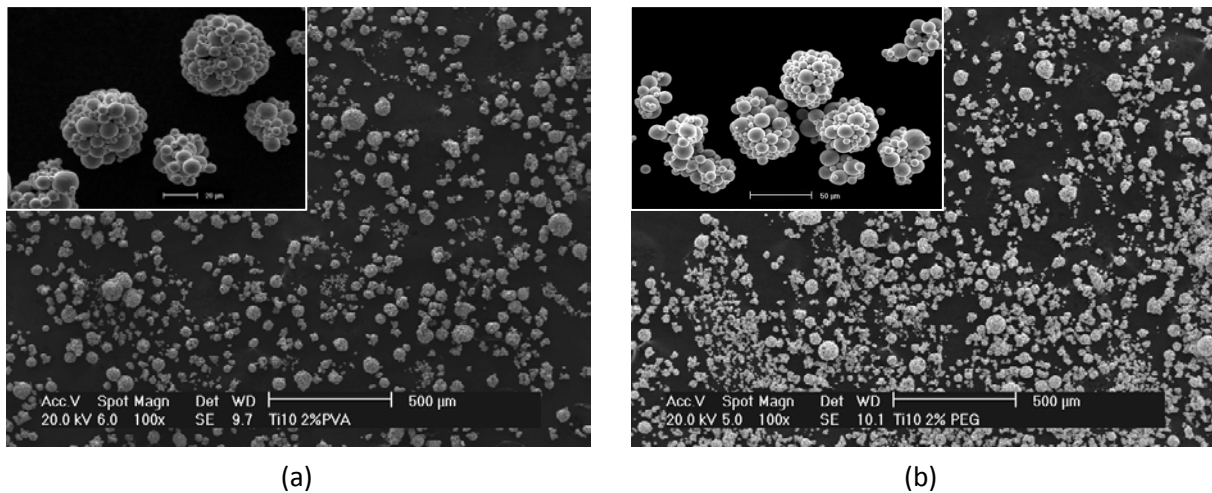
Figure 3- Granules obtained by Spray dry process for Ti10 µm [50% vol] with: a) 2% PVA b) 2% PEG. The compressibility of two powders, Ti45 and spray-dried Ti10 (as shown on figure 3.a), was studied by compacting samples at different pressures. Figure 4 shows the compressibility curves for these two powders. It can be observed that green density is higher for pressed Ti10 agglomerates than for Ti45 powder. This is due to the better particle size distribution and close packing that is achieved by employing the agglomerates. Once the pressure (600 MPa) was selected, samples were pressed and sintered at 1100 °C for 30 minutes.
