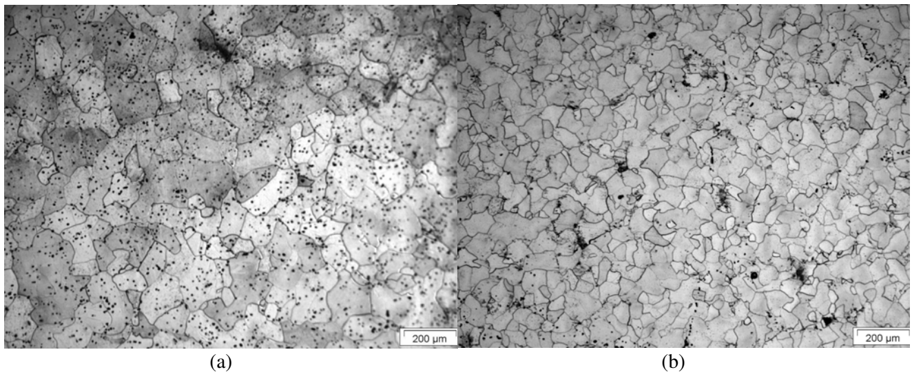
Figure 5. Microstructure of sintered samples obtained from (a) Ti45 as received powders and (b) Ti10 spray-dried powders, pressed and sintered in similar conditions.
