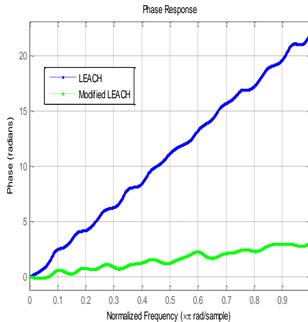
Fig 4: Phase recognition for Modified LEACH and LEACH
