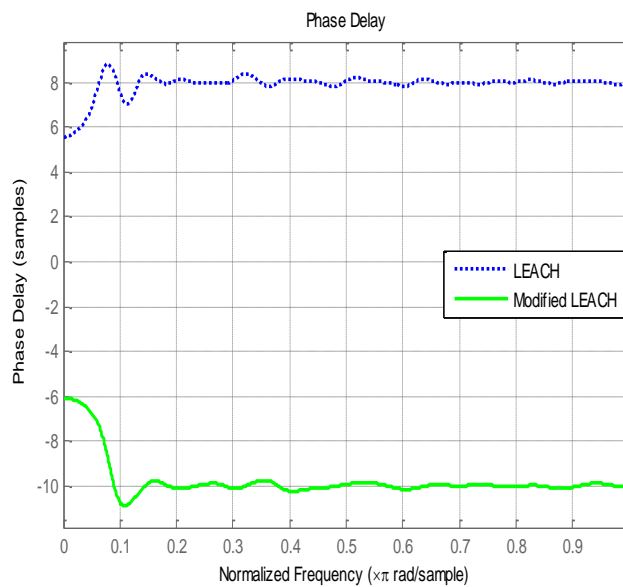
Fig 5: Phase delay between our protocol and LEACH
