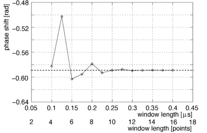
Fig. 5. Phase shift estimated at 7.5 MHz is plotted as a function of window length (with respect to simulated RF echoes, \tau_2 - \tau_1 = 12.5 ns).
