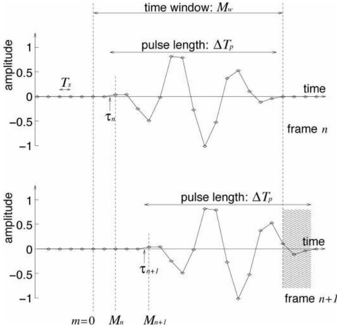
Fig. 1. Illustration of the change in relative position between the RF echo and the time window due to object displacement using simulated RF echoes.
