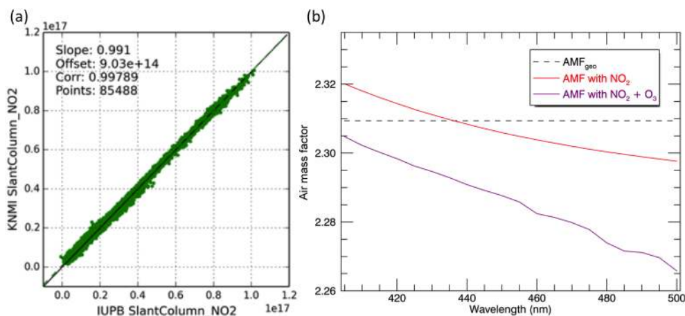
Figure 4. (a) Correlation plots of IUPB Bremen (425–497 nm fitting window) and KNMI (405–465 nm) NO 2 slant columns retrieved using preferred fit settings for OMI orbit OMIL2_2005m0202t0339, including only pixels with SZA < 88° and intensity < 1.1 × 10 14 . (b) Wave-length dependency of the total air mass factor for a scenario with SZA = VZA = 30° (geometrical AMF = 2.31), as calculated with DAK for a midlatitude standard atmospheric profile with a total NO 2 column of 5.9 × 10 15 molecules cm -2 (mostly situated in the stratosphere) (red curve), and for the same midlatitude standard atmospheric profile but now with absorption by both NO 2 and O 3 (total column of 322 DU, purple curve).
