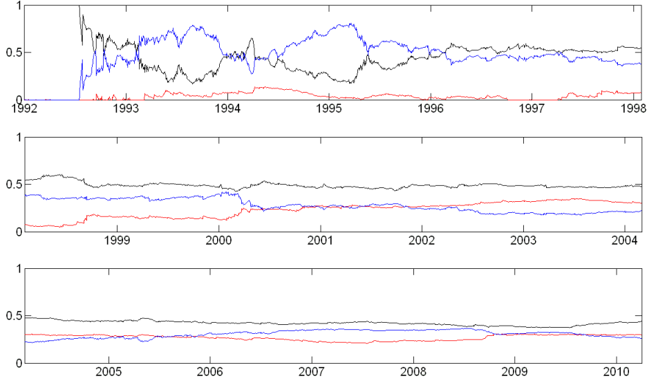
Figure 3: Optimal prediction pool weights, updated each trading day: sum of weights for daily models (black), high frequency models (red), and options models (blue).
