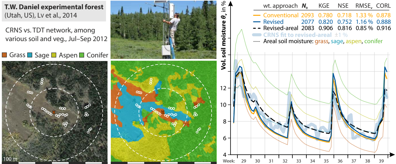
Figure 10. Time series of CRNS and TDT soil moisture at the T. W. Daniel Experimental Forest . The area was split into four categories (dotted lines), to which the corresponding soil moisture measurements were assigned. The areal coverage was then averaged (dashed line) pixel by pixel (1 m resolution) with the revised weighting approach, leading to the best performance against the CRNS signal.
