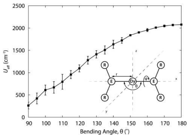
Fig. 9 Relaxation barrier U_{\text{eff}} for [Dy{N(SiH 3 ) 2 } 2 ] + as a function of the bending angle \theta , averaged for all torsion angles \phi . Structure of the model complex. Adapted with permission from ref. 21. Copyright 2015 American Chemical Society.
