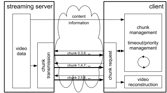
Fig. 3. Request-response-based client-driven streaming system
