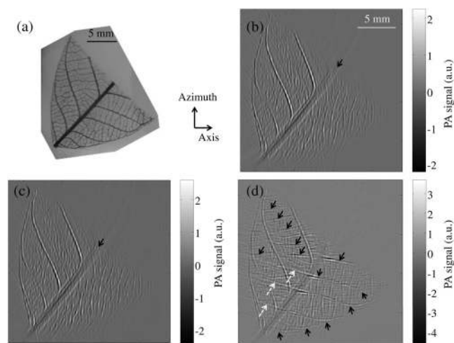
Fig. 3 PAT images of a leaf skeleton phantom. (a) Photo of the phantom. (b) Image of the leaf skeleton phantom acquired without the presence of the acoustic reflector. (c) Image of the phantom acquired with the presence of the reflector but reconstructed without incorporating data from the virtual array. (d) Image of the phantom acquired with the presence of the acoustic reflector and reconstructed with data from the virtual array incorporated.
