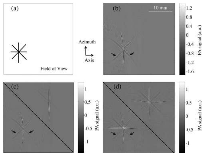
Fig. 2 Photoacoustic tomography (PAT) images of a hair phantom. (a) Diagram of the hair phantom; the gray rectangle indicates the approximate field of view. (b) Image of the hair phantom acquired without the presence of the acoustic reflector. (c) Image of the phantom acquired with the presence of the reflector but reconstructed without incorporating data from the virtual array. (d) Image of the phantom acquired with the presence of the reflector and reconstructed with data from the virtual array incorporated. The dashed line indicates the position of the acoustic reflector.
