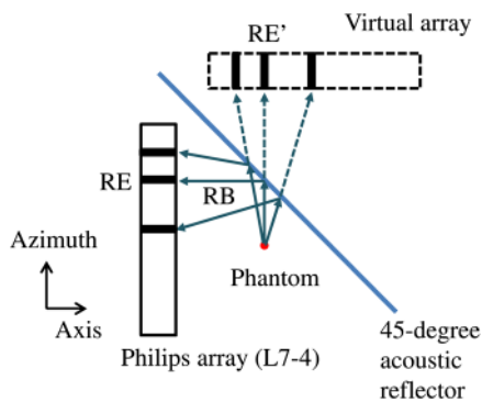
Fig. 1 Top view of the experimental setup. RB, reflected beam; RE, physical receiving element; RE', virtual receiving element. The commercial Philips array operated in B-mode to collect photoacoustic signals, a 45-deg acoustic reflector (glass) formed a virtual array, and a laser illuminated light orthogonally to the drawing from the top (not shown in the figure).
