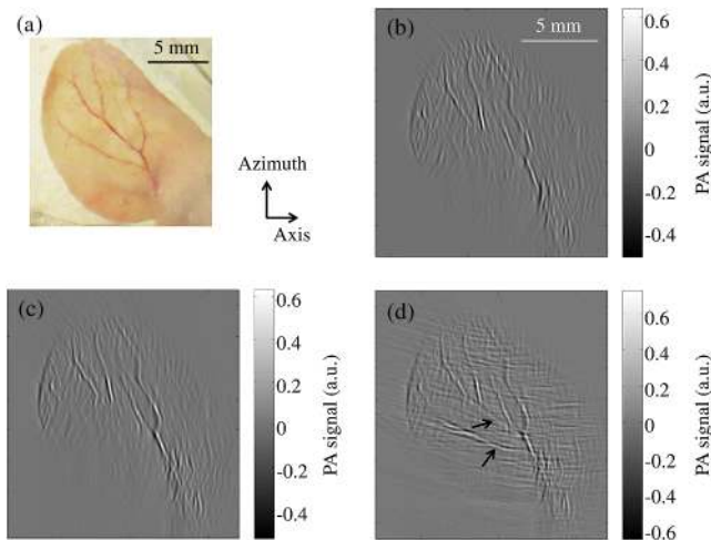
Fig. 4 Ex vivo PAT images of a mouse ear. (a) Photo of the mouse ear. (b) Image of the mouse ear acquired without the presence of the acoustic reflector. (c) Image of the mouse ear acquired with the presence of the reflector but reconstructed without incorporating data from the virtual array. (d) Image of the mouse ear acquired with the presence of the acoustic reflector and reconstructed with data from the virtual array incorporated.
