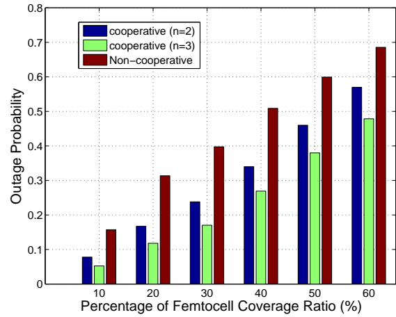
Fig. 10. Outage probability of the non-cooperative and cooperative schemes for various femtocell coverage ratios.
