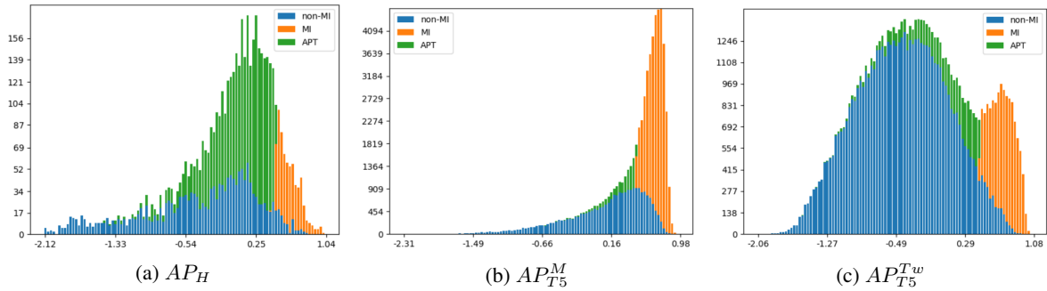
Figure 2: BLEURT distributions on adversarial datasets. All figures divide the range of observed scores into 100 bins. Note that APT sentence pairs are also MI , whereas those labeled ‘MI’ are not APT .
