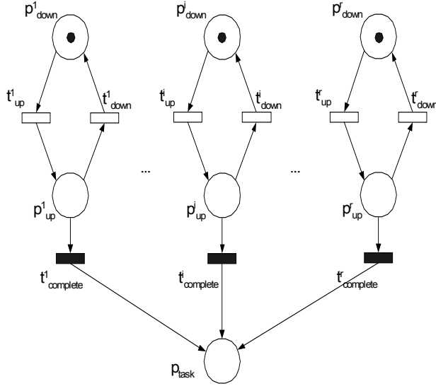
Figure 2: Petri Net Modeling of Computation Replication in the Grid
