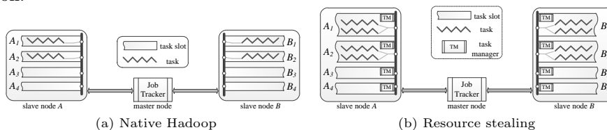
Fig. 1: Scheduling with native Hadoop and resource stealing
