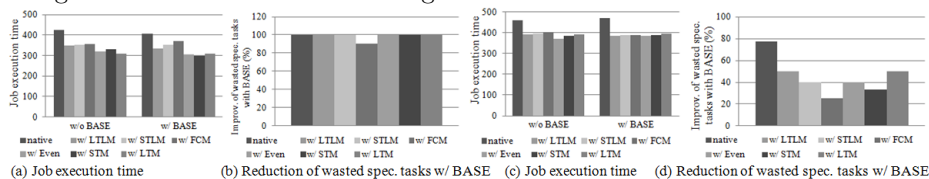
Fig. 3: Run map-only rep-grep with straggler nodes. There are two straggler nodes for (a) and (b), and four straggler nodes for (c) and (d)
