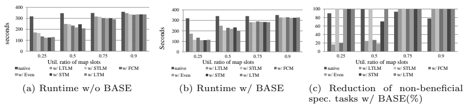
Fig. 2: Run map-only rep-grep in a homogeneous environment
