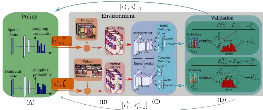
Fig. 1. (A) Deep RL of a policy for sampling permutations. (B) Permuting training images/videos by the proposed actions of (A) to provide self-supervision for our network architecture (C). (D) Evaluating the update network (C) on validation data to receive reward and state.
