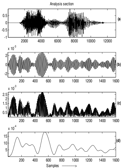
Fig 10. Uniform-bandwidth filters-based CI system - Analysis section (a) Input speech signal for the word 'sugar' (b) channel 5 output for the unvoiced region (c) corresponding full-wave rectified output and (d) envelope
