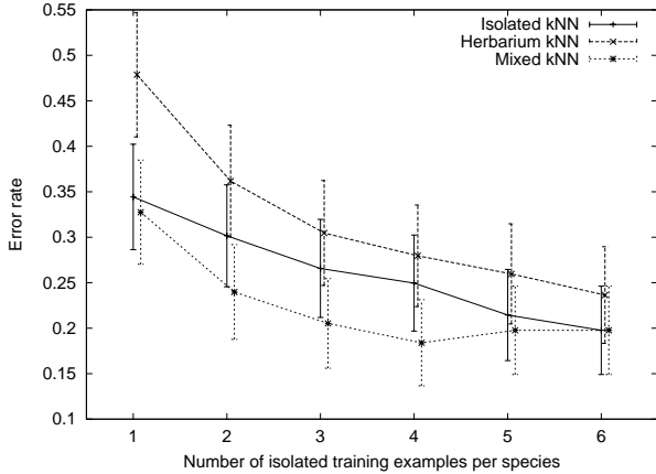
Figure 3. kNN error rates (error bars show 95% confidence interval)
