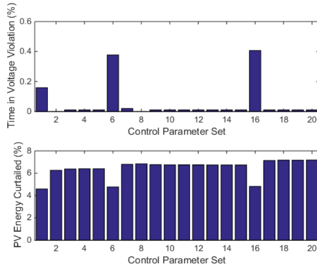
Figure 5.51. Comparison of sensitivity-based five-minute dispatch control parameter set performance.
