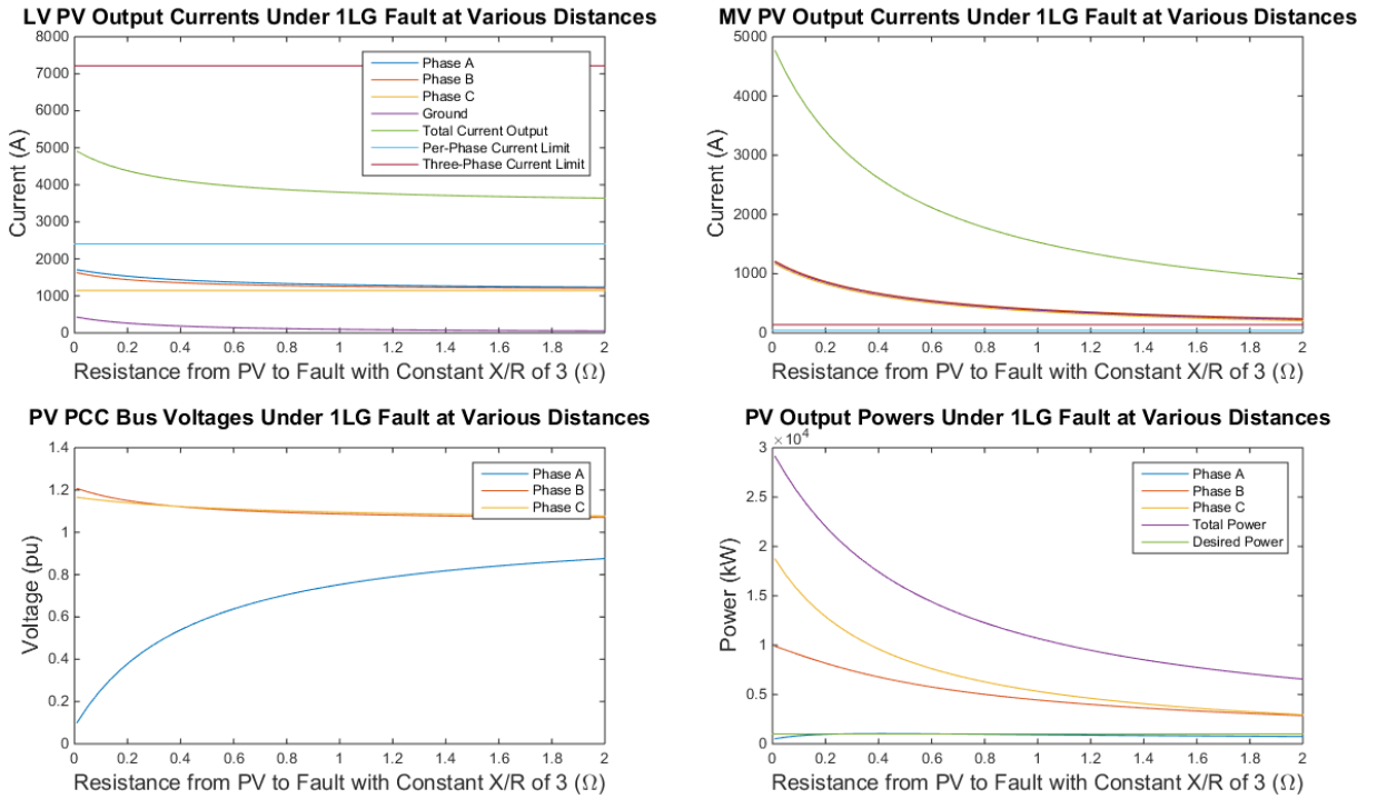
Figure B.1. Current-source PV output currents, power, and voltage using Y- \Delta interconnection transformer under 1LG faults.
