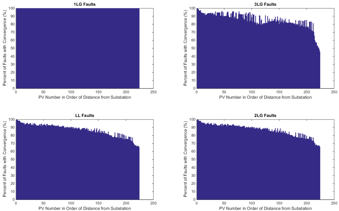
Figure A.5. Feeder QL2 percent of fault locations that result in convergence at largest PV size.
