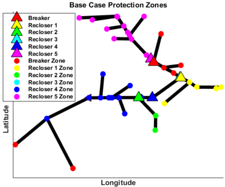
Figure 3.20. Feeder QW1 baseline protection zones colored by first PD to trip.
