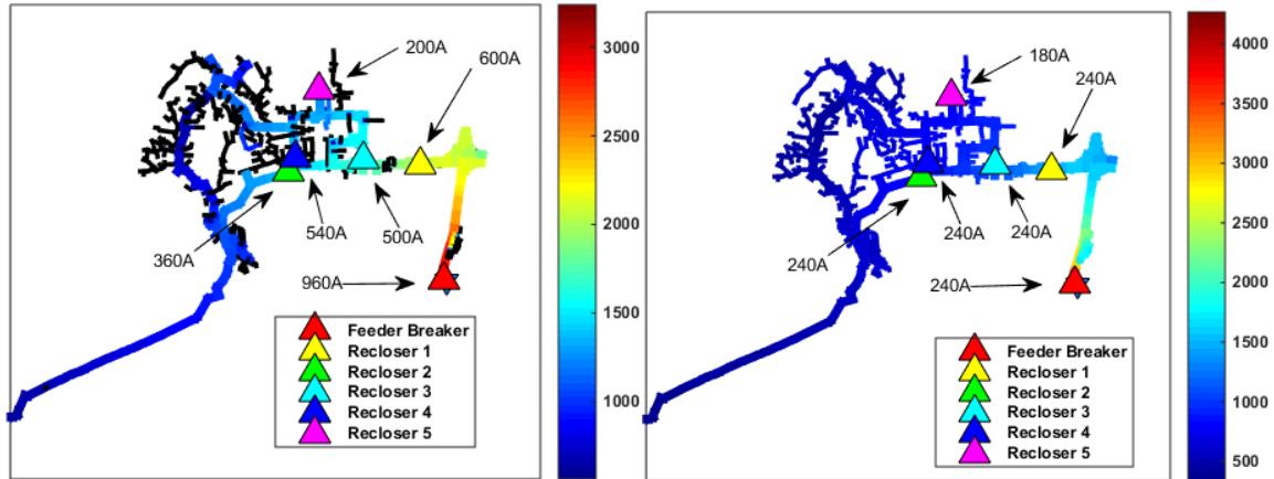
Figure 3.15. Feeder QL1 with the breaker and recloser a) minimum phase pickup current, and b) minimum ground pickup current. The lines are colored by the a) phase current for a 3LG fault and b) zero-sequence current for a 1LG fault at the bus.
