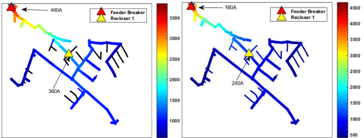
Figure D.6. Feeder QB1 with the breaker and recloser a) minimum phase pickup current, and b) minimum ground pickup current. The lines are colored by the a) phase current for a 3LG fault and b) zero-sequence current for a 1LG fault at the bus.
