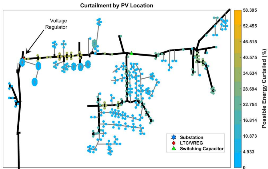
Figure 5.50. Zoomed-in section showing location of PVs curtailment more due to sensitivity-based dispatch control over the year than during worst week.
