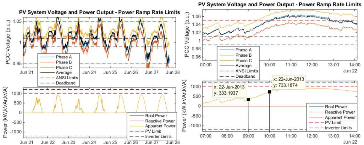
Figure F.1.(left) Power ramp-rate limiting applied to the PV inverter. (right) A zoomed-in segment of time showing ramp limiting.
