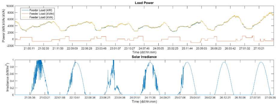
Figure 4.2. Weekly 1-minute resolution load and irradiance data selected for QSTS simulation to be representative of year.
