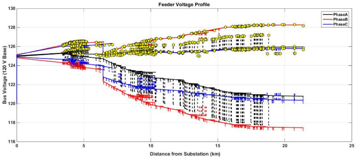
Figure 5.5. Feeder voltage profile at minimum load without PV and with PV, represented as yellow stars.
