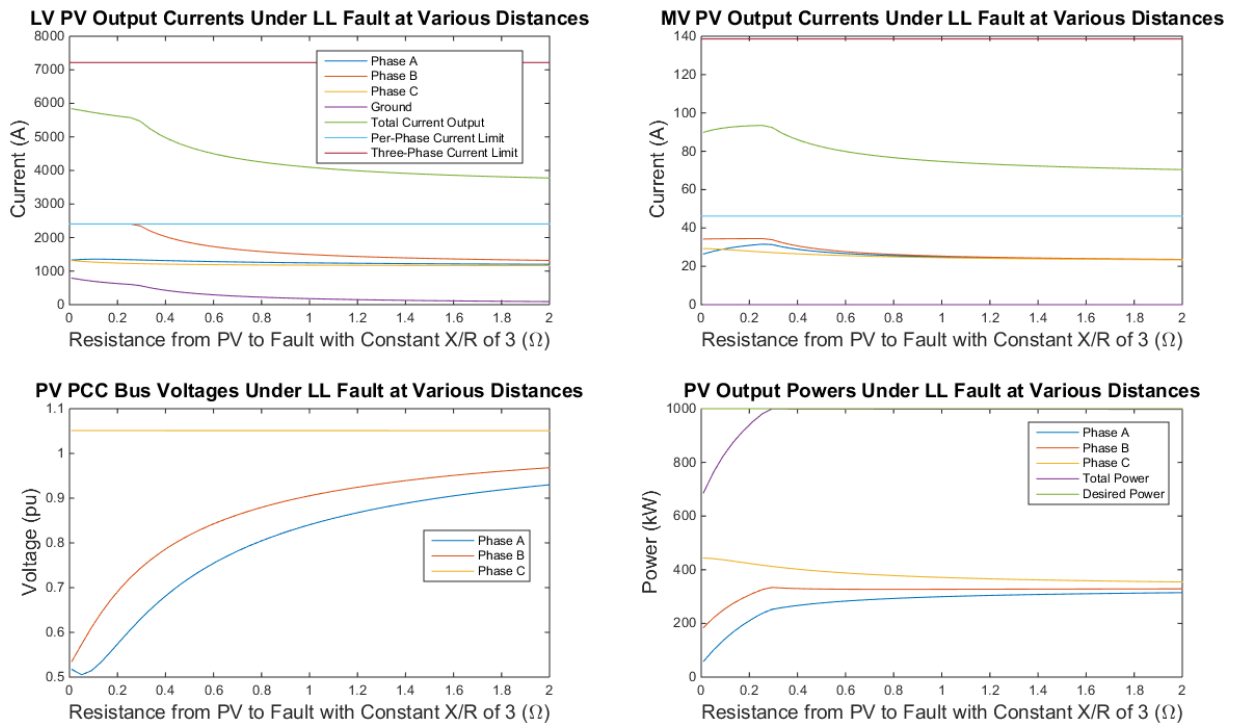
Figure B.2. Current-source PV output currents, power, and voltage using Y- \Delta interconnection transformer under LL faults.
