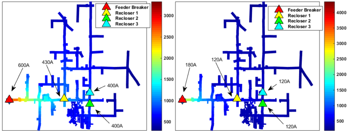
Figure 3.7. Feeder QS1 with the breaker and recloser a) minimum phase pickup current, and b) minimum ground pickup current. The lines are colored by the a) phase current for a 3LG fault and b) zero-sequence current for a 1LG fault at the bus.
