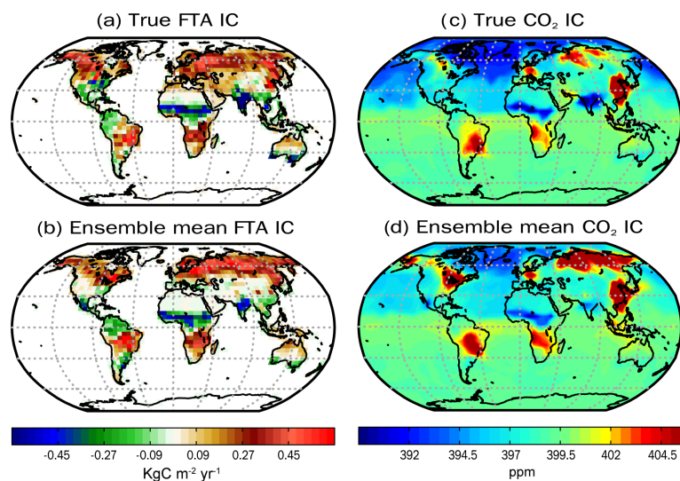
Figure A1. The initial FTA and surface CO 2 condition of the truth (a, c) and the ensemble mean first guess (b, d) on 1 October 2014.
