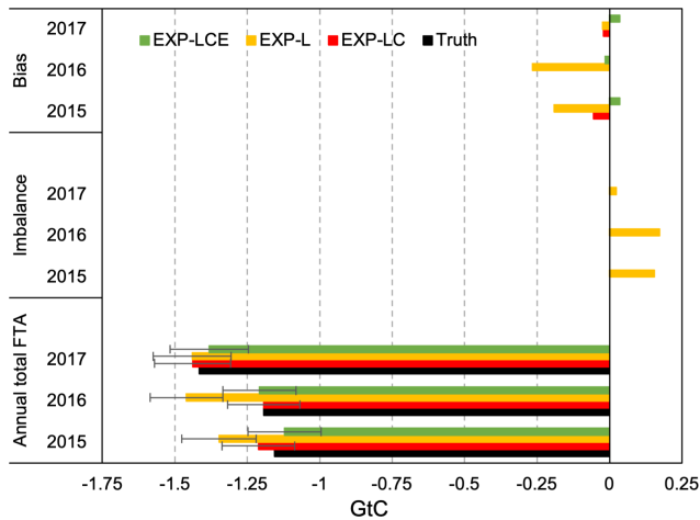
Figure 9. The global annual total FTA, imbalance, and bias of EXP-LC (red), EXP-L (orange), and EXP-LCE (green) compared with the truth (black) in 2015, 2016, and 2017. The imbalance is the mass loss for each year. The bias is the analysis of EXP-L and EXP-LC compared with the truth for each year. Note that there is no imbalance problem for EXP-LC and EXP-LCE. The error bar of the annual total is the uncertainty.
