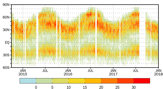
Figure 4. The daily pseudo OCO-2 land nadir and land glint observation numbers along the 4° latitude band.
