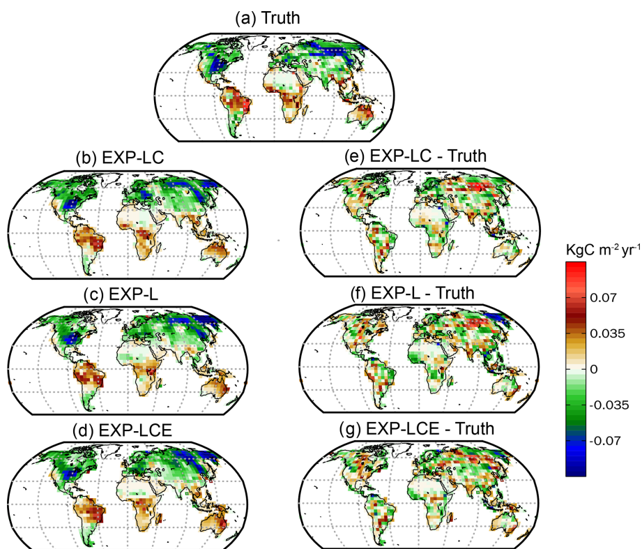
Figure 11. The spatial distribution of FTA for the truth (a), EXP-LC (b), EXP-L (c), and EXP-LCE (d) averaged from January 2015 to December 2017. The annual mean of the prior FTA is not shown because it is zero at each grid. The bias of EXP-LC compared with the truth (e), EXP-L compared with the truth (f), and EXP-LCE compared with the truth (g).
