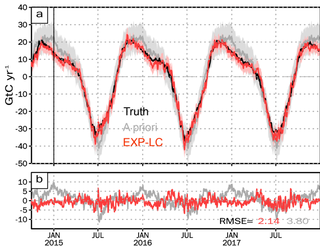
Figure 5. (a) The global daily FTA of truth (black), a priori (gray), and analysis of EXP-LC (red). The vertical line on 1 January 2015 indicates the start of assimilation. Before 1 January 2015, the system spin-up lasted for 3 months. The pale gray and pale red shadings are the ensemble spread of the a priori and analysis, respectively. (b) The difference compared with the truth. The RMSE at the bottom right corner is the root mean square error of the analysis (red) and the a priori (gray) calculated based on Eq. (12).
