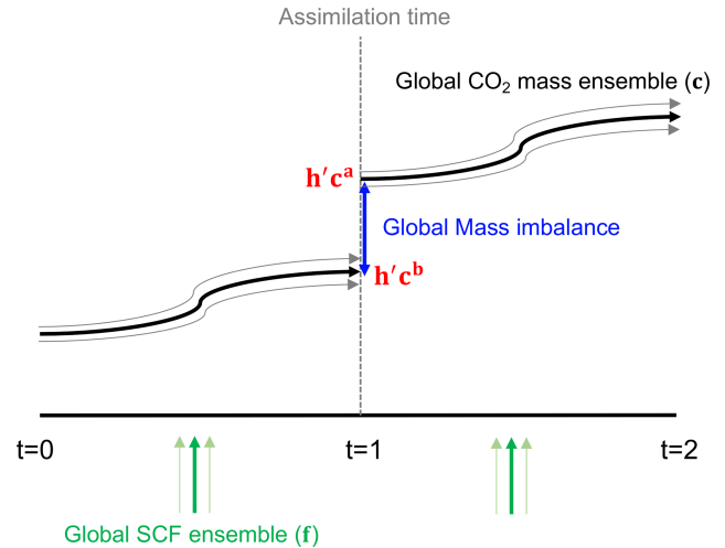
Figure 2. Schematic illustration of the mass imbalance problem.
