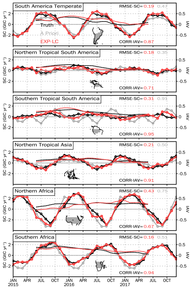
Figure 7. Same as in Fig. 6 but for the tropical regions.
