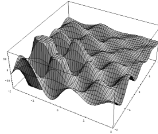
Figure 3.1 The original plot of the function Levy No. 5 .
