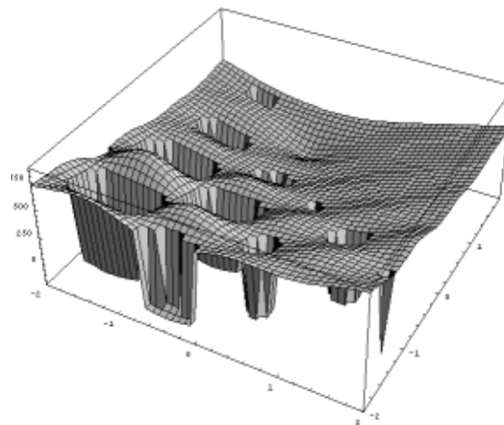
Figure 3.2 Plot of the Levy No. 5 after the first stage of the “Stretching” technique.
