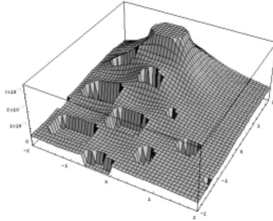
Figure 3.3 Plot of the Levy No. 5 after the second stage of the “Stretching” technique.
