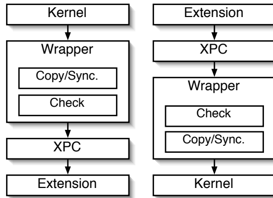
Fig. 4. Control flow of extension and kernel wrappers.
