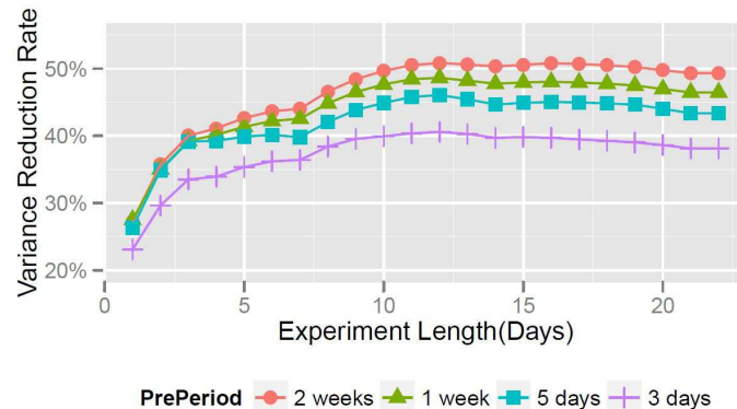
Figure 4: Impact of pre-experiment period length.
