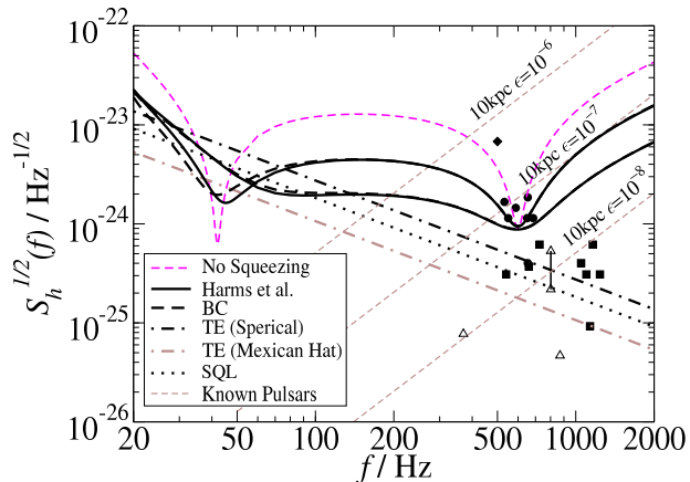
FIG. 7: Noise curves of non-squeezed (light dashed curve), Harms et al. (dark continuous curves) and BC (dark dashed curves) configurations optimized for narrowband sources, for 5 dB and 10 dB squeezing. We apply only one filter, that is the one with resonant frequency near the free optical resonant frequency of the SR interferometer, or filter I (see Table V). The interferometer noise curves contain only quantum noise but include filter losses. The thermoelastic noise of spherical and MH mirrors, and the SQL are plotted for comparison. We also show the frequencies and characteristic strengths (20-day coherent integration, 1% false alarm [38, 39]) of possible GWs from LMXBs [41] [using the baseline assumption (a1), namely f_s = f_d and mass-quadrupole emission]: Z sources in solid circles (Sco X-1 in diamond), Type-I X-ray bursters in solid squares and accreting millisecond pulsars in open triangles. For the accreting millisecond pulsar SAX J1808.4-3658, for which the orbital parameters and GW phase evolutions are known [45], we show in another open triangle (linked to the 20-day one with a vertical segment of solid line) the characteristic strength assuming a 4-month integration.
