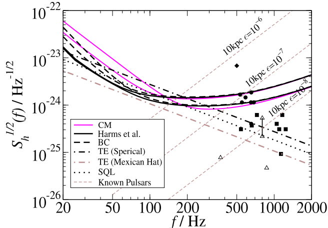
FIG. 10: Noise spectral densities of wideband configurations, with \epsilon = 2\pi \times 600 Hz and \lambda = 0 , frequency-independent squeezing ( \alpha = \pi/2 , \zeta = 0 , light continuous curve), the Harms et al. scheme ( \zeta = 0 , dark continuous curve) and the BC scheme ( \alpha = \pi/2 , dark dashed curve) are used. Only the quantum-optical noise (taking filter losses into account) is included. Thermoelastic noises of spherical and MH mirrors are also shown, in dark and light dash-dot lines, respectively. The SQL is shown in dashed line. Possible GW signals from LMXBs [under the baseline assumption] and known radio pulsars are also shown.
