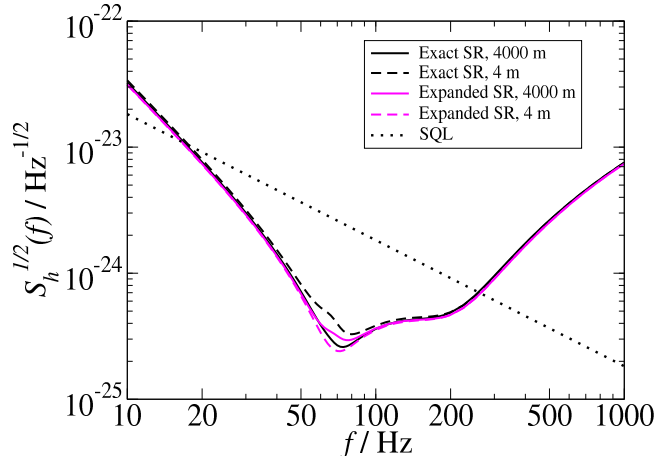
FIG. 14: To investigate the short-filter and short-arm approximation in SR squeezed-variational interferometers we plot several noise curves fixing I_c = 840 kW, m = 40 kg, e^{-2r} = 0.1 , \epsilon = 2\pi \times 80 Hz and \lambda = 2\pi \times 200 Hz. In particular we show the noise curve obtained with exact input-output relation and 4 km filter cavities (dark continuous curve), and 4 m filter (dark dashed curve); the noise curves obtained with first-order expanded input-output relation and 4 km filter (light continuous curve) and 4 m filter (light dashed curve). We use T_e = 20 ppm for the 4 km configurations, and T_e = 0.02 ppm for 4 m configurations, such that the overall loss factor remains the same. The disagreements between curves with the same pattern (continuous or dashed) but different color (dark or light) is due to the inaccuracy of short-filter approximation; while the disagreements between curves with the same color but different pattern is due to the inaccuracy of short-arm approximation.
