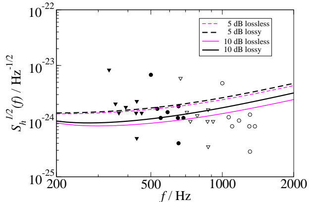
FIG. 12: Consequences of spin-frequency and emission-mechanism uncertainties on the detection of LMXBs (Z sources) using the wideband configuration. We plot the GW frequency and characteristic GW strength (for 20-day coherent integration), under approximations (a1) (solid circles), (b1) (open circles), (a2) (solid triangles) and (b2) (open triangles), along with CM noise curves with 5 dB (dashed curves) and 10 dB (continuous curves) squeezing, with (dark curves) and without (light curves) interferometer losses.
