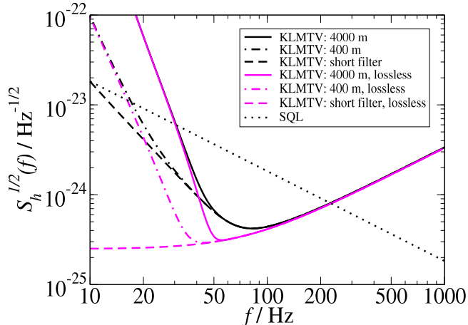
FIG. 13: To show the break-down of the short-cavity approximation we plot several noise curves for the KLMTV (conventional) squeezed-variational interferometer [20] with I_c = 840 kW, m = 40 kg and e^{-2r} = 0.1 , fixing a bandwidth of \epsilon = 2\pi \times 75 Hz. The dark continuous curve refers to the nominal filter-cavity length L_f = 4 km, and the round-trip filter loss T_e = 20 ppm; while the short-filter approximation ( L_f = 0.1 m) predicts the dark dashed curve. For comparison, we also plot noise curves of configuration with L_f = 400 m, T_e = 2 ppm (dark dash-dot curve), along with those of the lossless optical configurations with L_f = 4 km (light continuous curve), L_f = 400 m (light dash-dot curve) and with short-filter approximation ( L_f = 0.1 m) (light dashed curve).
