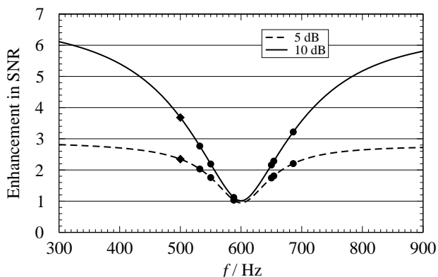
FIG. 8: Relative increase in SNR for LMXB sources around 600 Hz, with 5 dB ( e^{-2r} = 0.316 , dashed curve) and 10 dB ( e^{-2r} = 0.1 , continuous curve) squeezing. Since the Harms et al. and BC schemes are extremely close to each other only one curve is shown for each squeeze factor. The various detectable LMXBs [under the baseline assumption] listed in Table V are also shown (Sco X-1 in solid diamond, the rest in solid circles)
