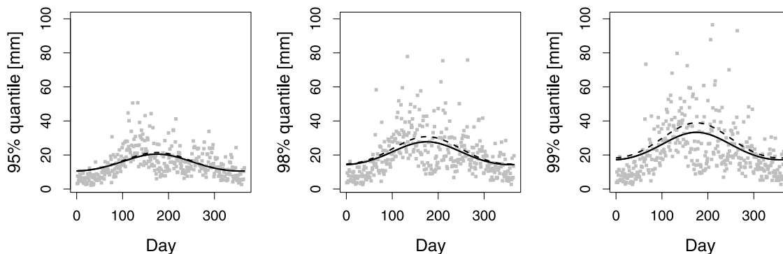
Figure 9. High quantiles of fitted gamma (solid lines) and hybrid gamma/GP (dashed lines) distributions as functions of the day of year for Fort Collins precipitation intensity. Empirical quantiles calculated from the 100 years of observed precipitation are shown as dots.
