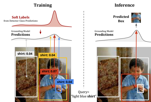
Figure 1: Our method uses object detector predictions to guide the learning of region-phrase matching in training. At the inference time, our method no longer requires object detectors and directly predicts the box with the highest score.
