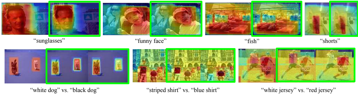
Figure 3: Visualization of region-phrase matching. First row: results of the NCE only (left) and the NCE+Distill (green) on phrases mapped to Open Images Dataset classes. Second row: results of the Distill only (left) and NCE+Distill (green) on phrases mapped to the same class but with different attributes. For each pixel, we compute a matching score by averaging scores from all proposals covering the pixel. Red colors indicate high matching scores. Our knowledge distillation helps to better identify the extent of objects, while contrastive learning helps to distinguish finer attributes.
