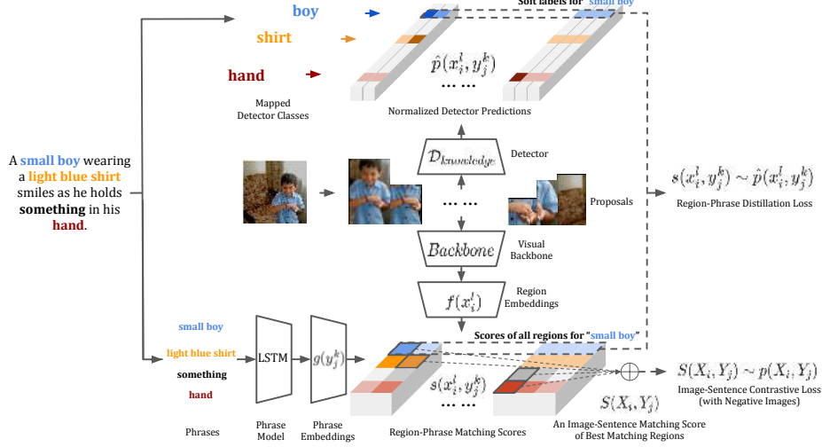
Figure 2: Overview of our method in training. A contrastive learning framework is designed to account for both region-phrase and image-sentence matching. The top part illustrates region-phrase matching learned by distilling from object detection outputs, while the bottom part shows image-sentence matching supervised by ground-truth image-sentence pairs.
