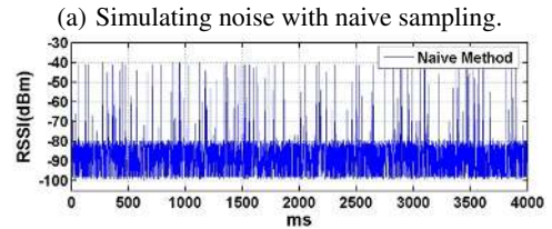
(a) Simulating noise with naive sampling. (b) Sample noise trace from naive sampling using heavy traffic Meyer trace.
