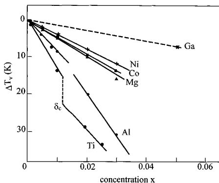
FIG. 4. The shift of the Verwey transition temperature for substituted stoichiometric magnetites \text{Fe}_{3-x}\text{M}_x\text{O}_4 , with M=\text{Ga}, \text{Ni}, \text{Co}, \text{Mg}, \text{Al}, and \text{Ti} . The Ti data are from Refs. 26 and 31 ( x=0.003 and 0.008 ).
