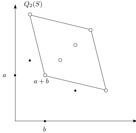
Figure 2: A set S_2 of 4 points in \mathbb{R}^2 (black) and the corresponding 2-set polytope.
