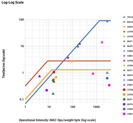
Figure 8. Figures 5-7 combined into a log-log graph. Stars are for the TPU, triangles are for the K80, and circles are for Haswell. All TPU stars are at or above the other two rooflines.
