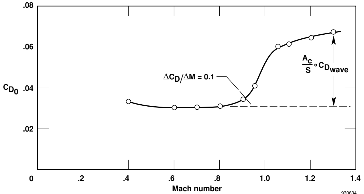
Figure 14. Variation of zero-lift-drag coefficient with Mach number and illustration of transonic wave drag increment; trimmed flight, ACC mode.
