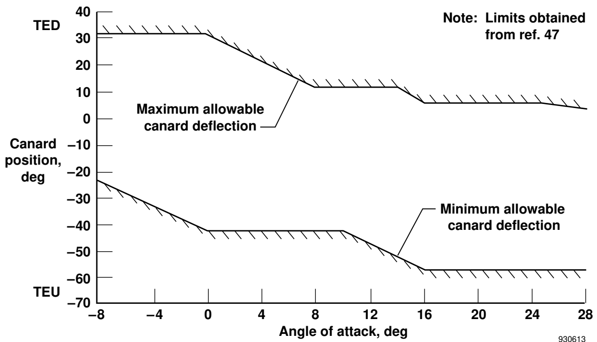
(a) Canard.
