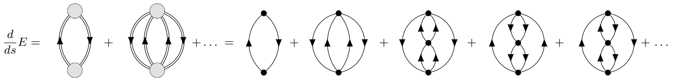
FIG. 2. Schematic illustration of the energy flow equation (14) for the White generator (20) in terms of Hugenholtz diagrams (see text). The grey vertices correspond to H(s) , and the double lines indicate energy denominators calculated with f(s) . On the right-hand side, the flow equation is expanded in terms of H(s - \delta s) (simple black vertex) and the corresponding energy denominators from f(s - \delta s) (single lines). The dots indicate omitted terms from the expansion of the Epstein-Nesbet energy denominator, as well as additional diagrams generated by the integration step s - \delta s \rightarrow s .
