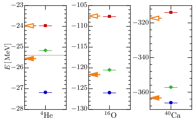
FIG. 6. (Color online) Ground-state energies of stable closed-shell nuclei for the bare NN Hamiltonian ( \lambda = \infty ), using IM-SRG(2) (●), CCSD (■), and \Lambda -CCSD(T) (◆). IM-SRG and CC results are obtained with \epsilon_{\text{Max}} = 14 . The gray solid line for {}^4\text{He} indicates the result of a converged NCSM calculation, E = -25.39 MeV (see e.g. [4]). The open and solid orange arrows are converged CCSD and \Lambda -CCSD(T) results from [38, 39].
