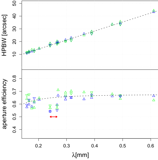
Fig. 3. HPBW and aperture efficiencies observed as a function of wavelength towards the planet Mars. Blue and green symbols represent observed values for horizontal and vertical polarization, respectively, whereas up and down pointing triangles distinguish two different observing runs. The black dashed lines represent fits to the relations described by Eqs. 3 and 1, resp. Observations in band 5 (marked with the red arrow) were excluded from the fit to the aperture efficiencies.
