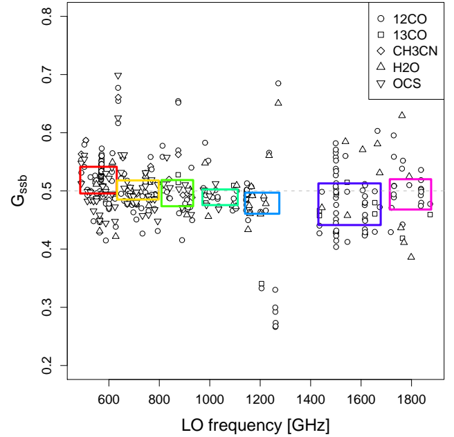
Fig. 1. Normalized sideband gain as a function of LO frequency and mixer bands (different colors)– G_{ssb} = 0.5 corresponds to equal gain in USB and LSB. The different gases used are indicated by the different symbols: ^{12}\text{CO} circles; ^{13}\text{CO} squares; \text{CH}_3\text{CN} diamonds; \text{H}_2\text{O} upward pointing triangles; OCS downward pointing triangles. Measurements in horizontal polarization have a black outline. The filled boxes delineate all data falling within the first and third quartiles. See text for caveats.
