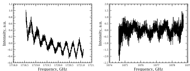
Fig. 4. Examples of the 320 MHz standing wave seen in the HEB IF chain (left panel) and the 680 MHz standing wave due to reflection between the mixer focus and the diplexer rooftop mirror (right panel)
