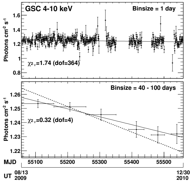
Fig. 11. (Top) Crab nebula light curve by GSC in 4–10 keV band in one-day time bin. The vertical errors represent the 1\text{-}\sigma statistical uncertainties. Solid line represents the best-fit linear model. The reduced chi-square ( \chi^2_{\nu} ) and the degrees of freedom (DOF) of the fit is shown on the panel. (Bottom) The same Crab nebula light curve but in 40–100-day time bin and the best-fit linear model. The model with a slope extrapolated from the 5.1% decline from MJD 54690 to 55435 observed by RXTE/PCA in 2–15 keV band (Wilson-Hodge et al. 2011) is shown together with dashed line.
