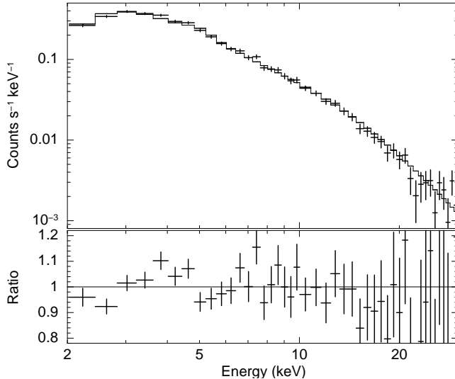
Fig. 12. GSC Crab-nebula spectrum taken for a day on August 15, 2009 (UT) and the best-fit power-law model with a fixed absorption of 0.35 \times 10^{22} \text{ cm}^{-2} (top). Data-to-model ratio (bottom).
