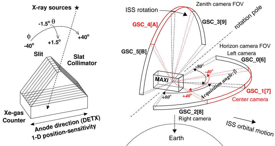
Fig. 1. (Left): Schematic view of a single GSC camera unit and its field of view (FOV) of 1.5^\circ (FWHM) \times 80^\circ . (Right): FOVs of the six camera units including 12 counters (GSC_0, ..., GSC_9, GSC_A, GSC_B) on the ISS low-earth orbit. Every two counters, such as GSC_0 and GSC_6, are used as a pair for a redundancy. Left, center, and right camera units cover the area of source-acquisition angle \beta of -80^\circ < \beta < 0^\circ , -40^\circ < \beta < +40^\circ , and 0^\circ < \beta < +80^\circ , respectively.
