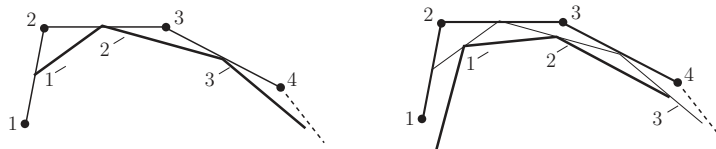
FIGURE 1. Iterations of Buffon transformations.
