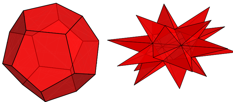
FIGURE 5. The dodecahedron and affine great stellated dodecahedron.
