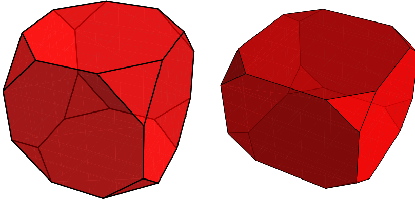
FIGURE 6. The truncated cube and affine B -regular truncated cube.
