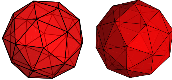
FIGURE 9. The pentakis dodecahedron and its affine B -regular version.
