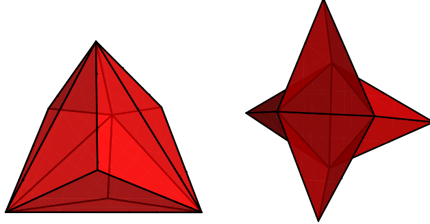
FIGURE 7. Triakis tetrahedron and its affine B -regular version, which is star-shaped but not convex.
