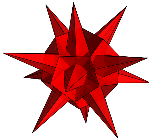
FIGURE 10. Eigenspace realisation corresponding to \lambda_8 = (60 + 5\sqrt{5} - \sqrt{725 + 240\sqrt{5}})/120 conjugated to \lambda_2 . The pyramids are built inside and go through the dodecahedron.
