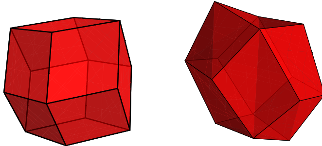
FIGURE 8. The rhombic dodecahedron and the corresponding subdominant eigenspace realisation: all the faces are broken (non-planar).
