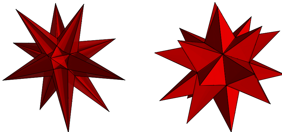
FIGURE 11. Eigenspace realisations corresponding to two remaining multiplicity 3 eigenvalues \lambda_4 and \lambda_9 : great icosahedron and great stellated dodecahedron with extra vertices.
