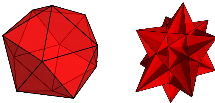
FIGURE 4. The icosahedron and affine great icosahedron.
