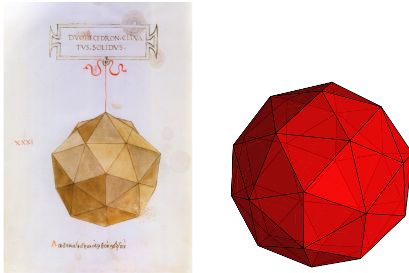
FIGURE 2. Leonardo da Vinci's drawing of pentakis dodecahedron from Luca Pacioli's book "De divina proportione" and Mathematica image of its Buffon realisation. Leonardo's version is different both from Catalan and Buffon realisations and probably corresponds to the so-called cumulated dodecahedron having all the edges of equal length.
