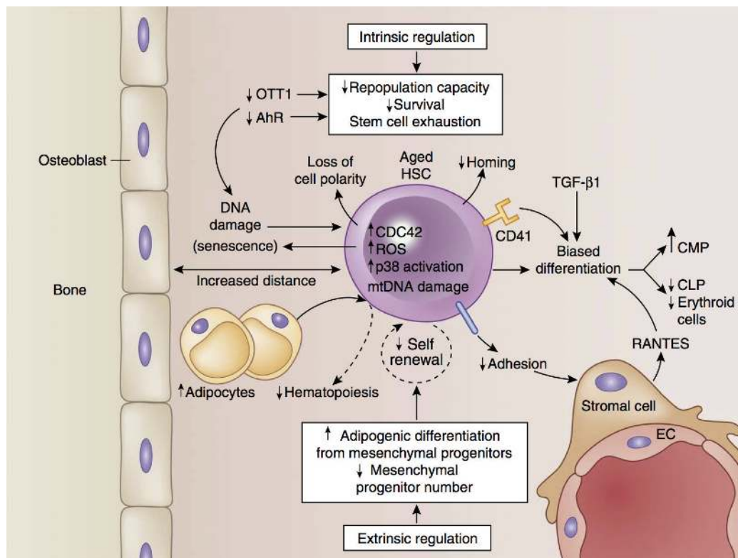
Figure 4. The effects of aging on HSC behavior.(74) (Adapted with permission from Nature Publishing Group).
