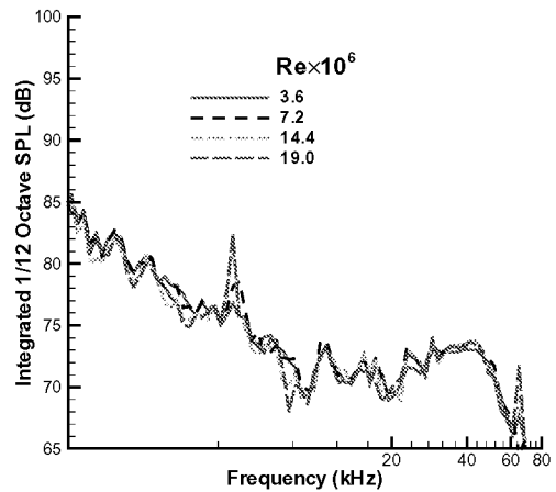
Fig.4 Measured acoustic spectra for EET slat at 20 deg deflection with M=0.2 . Reynolds number is based on stowed chord and frequencies are model scale frequencies.
