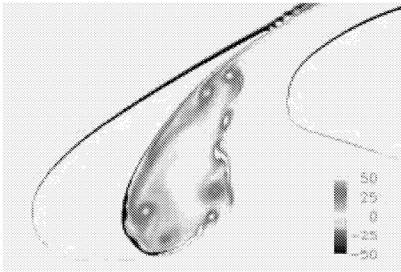
Fig. 11 Simulated instantaneous spanwise vorticity field for partially laminar-cove case. Flow conditions are same as for Fig.10.
