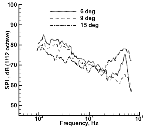
Fig. 9 Variation of measured slat noise with angle of attack at M=0.2 and Re_c=7.2 million. Slat deflection is 30 deg.
