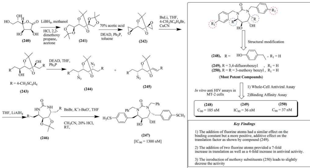
Fig. 32 Synthesis of P1/P1'-substituted cyclic urea-based derivatives together with important key findings of most potent compounds (248–250).
