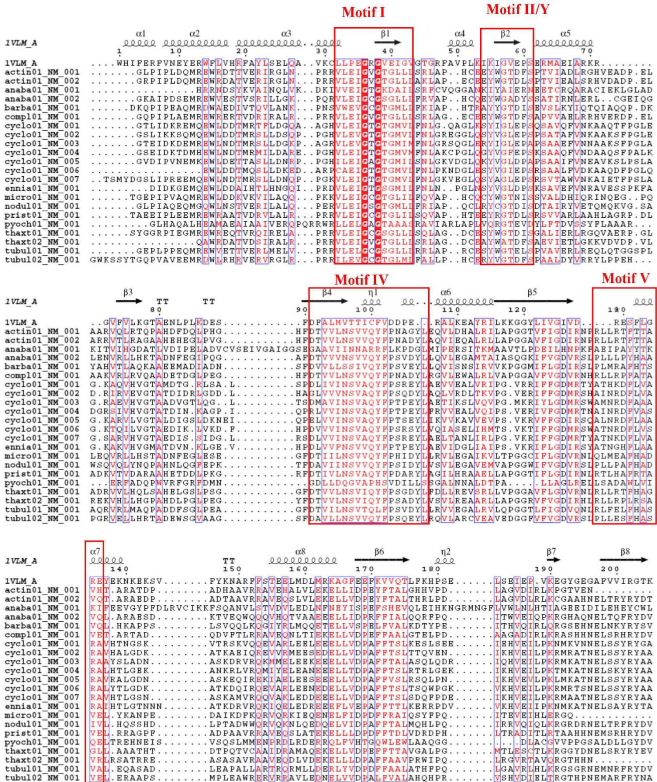
Figure 5 Multiple sequence alignments of N-MT domains from experimentally characterized NRPS/PKS clusters with the structural template IVLM.
