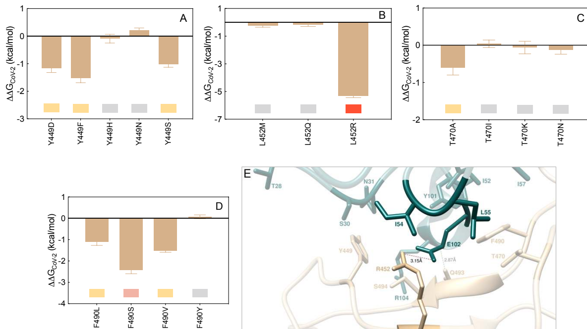
Figure 8. Change in binding free energy ( \Delta\Delta G = \Delta G_{\text{WILD-TYPE}} - \Delta G_{\text{MUTANT}} ) predicted by computational mutagenesis of the S-RBD CoV-2 wild-type residues Y449 (A), L452 (B), T470 (C) and F490 (D) for the corresponding S-RBD CoV-2 /LY-CoV555 mAb complexes. Colors and other explanations as in Figure 4. The numerical values of \Delta\Delta G , all related energy terms, and all underlying intermolecular intramolecular interactions are reported in Table S4, Figures S7-S10, and Tables S11-S14. (E) Main interactions involving the S-RBD CoV-2 L452 R mutant at the interface with the LY-CoV555 (bamlanivimab) mAb as obtained from the relevant
