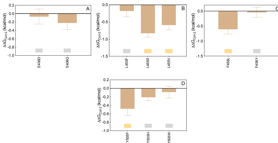
Figure 15. Change in binding free energy ( \Delta\Delta G = \Delta G_{\text{WILD-TYPE}} - \Delta G_{\text{MUTANT}} ) predicted by computational mutagenesis of the S-RBD CoV-2 wild-type residues E406 (A), L455 (B), F456 (C) and Y505 (D) for the corresponding S-RBD CoV-2 /LY-CoV016 mAb complexes. Colors and other explanations as in Figure 4. The numerical values of \Delta\Delta G , all related energy terms, and all underlying intermolecular intramolecular interactions are reported in Table S18, Figures S19-S22 and Tables S27-S30.
