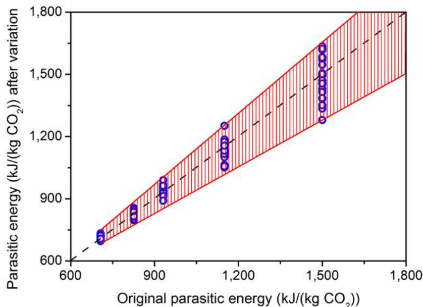
Figure SI 1: Uncertainties in the estimates of the parasitic energies. The blue dots are the 25 parameters sets for which we recalculated the parasitic energy after a change of +/- 20% of all parameters. The red line gives the upper and lower bounds of the errors in these sets.
