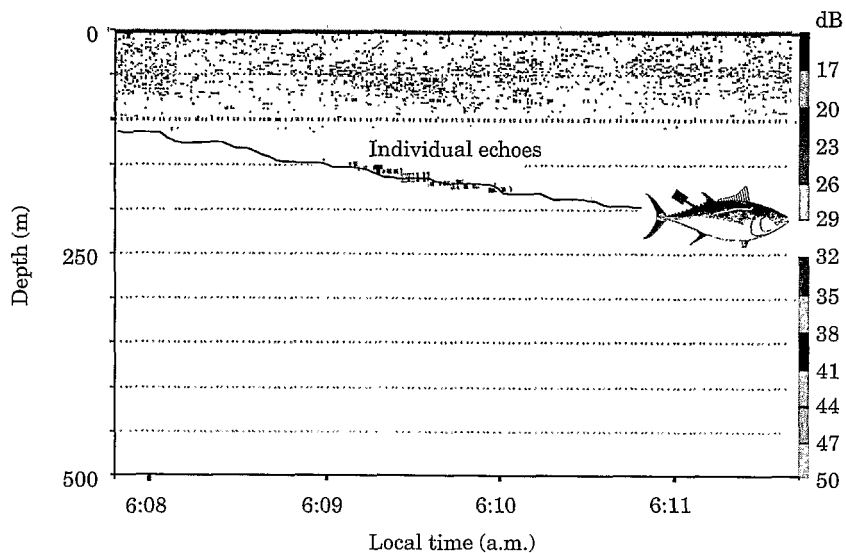
Figure 1. Echoes (points) and depth (solid line) of a tracked fish.
